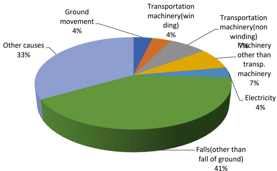
Fig. 3 Cause-wise distribution of fatal accidents in metalliferous mines during 2023
