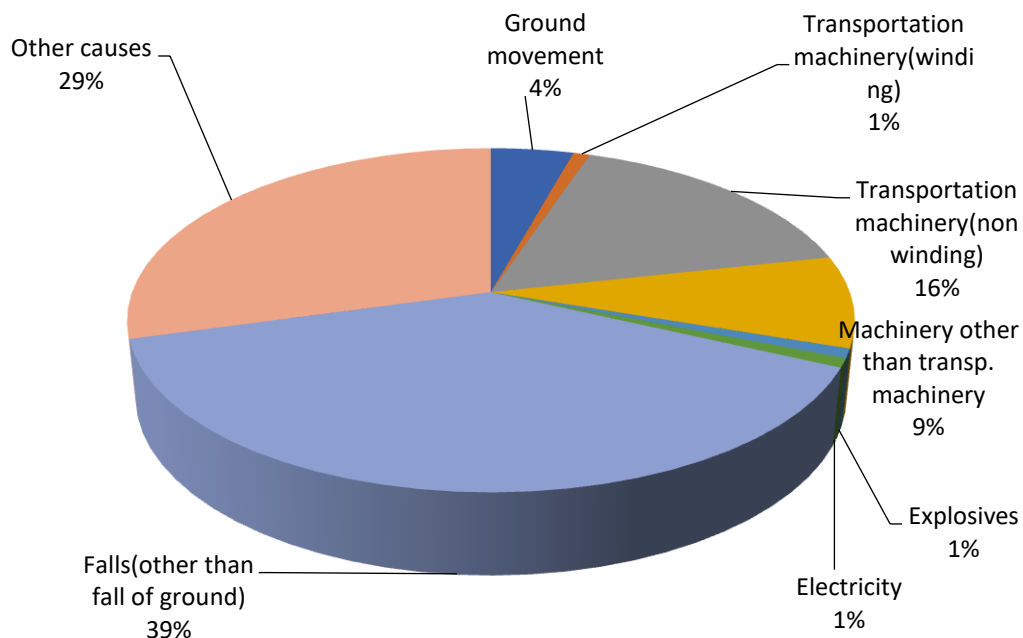
Fig.2 Cause-wise distribution of serious accidents in coal mines during 2023
