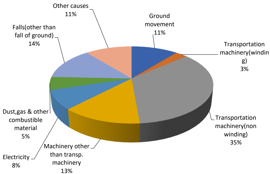
Fig.1 Cause-wise distribution of fatal accidents in coal mines during 2023
